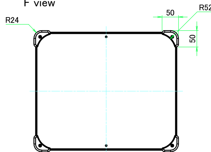
F view
