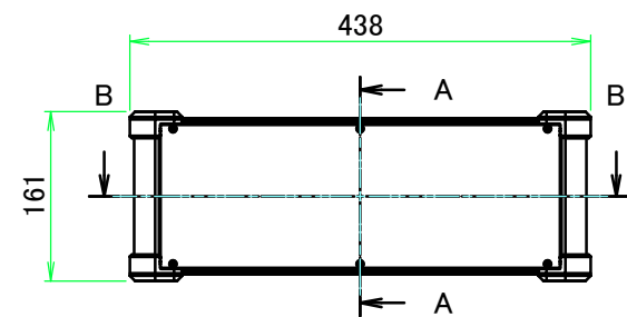
A view
