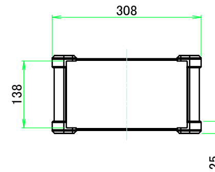
C view
