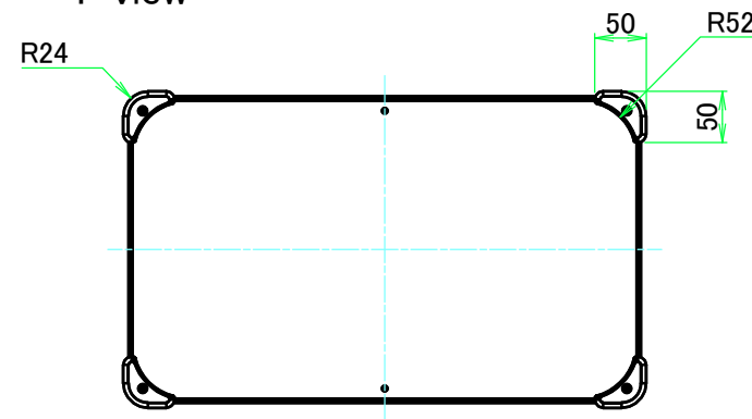
F view
