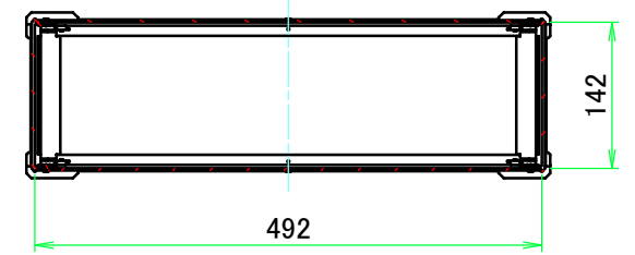
C-C (1:8)
