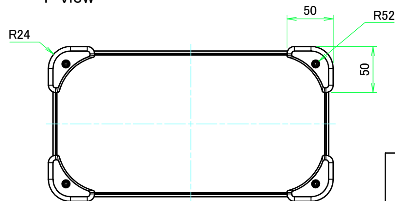
F view
