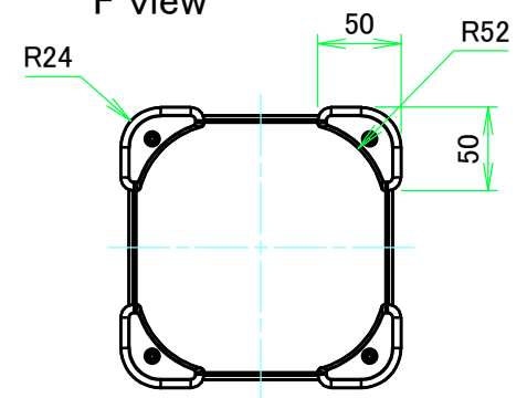
F view
