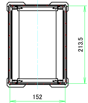
B view
