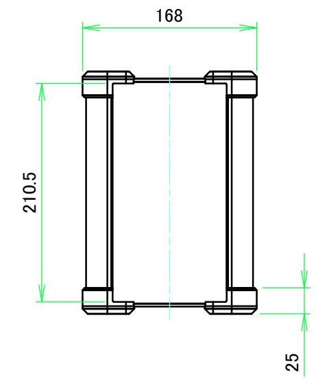
C view
