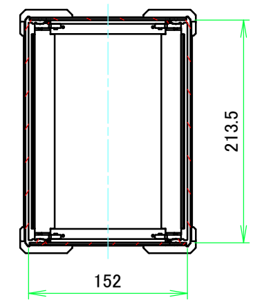
C-C (1:5)
