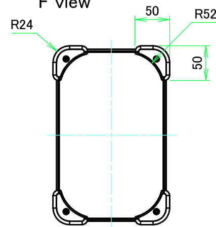
F view
