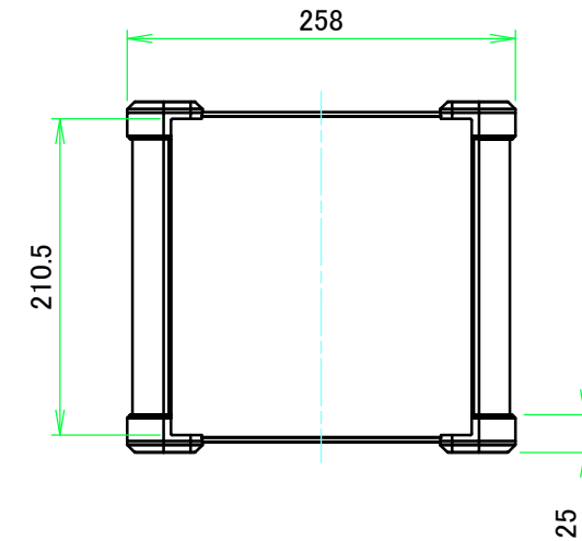
C view
