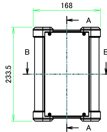
A view
