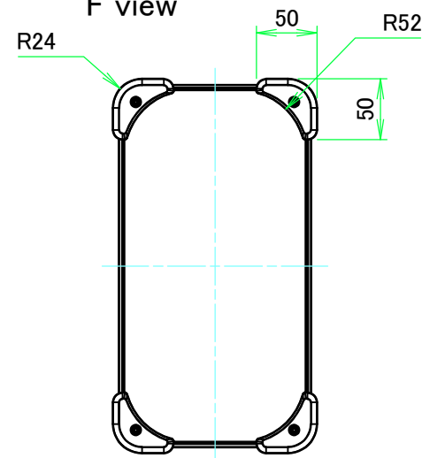
F view
