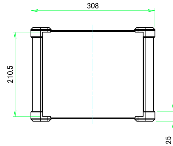
C view
