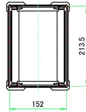
C-C (1:6)
