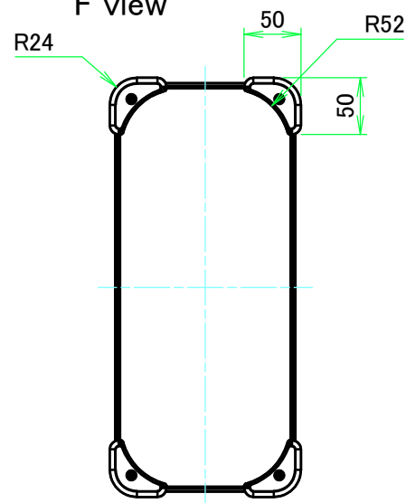
F view
