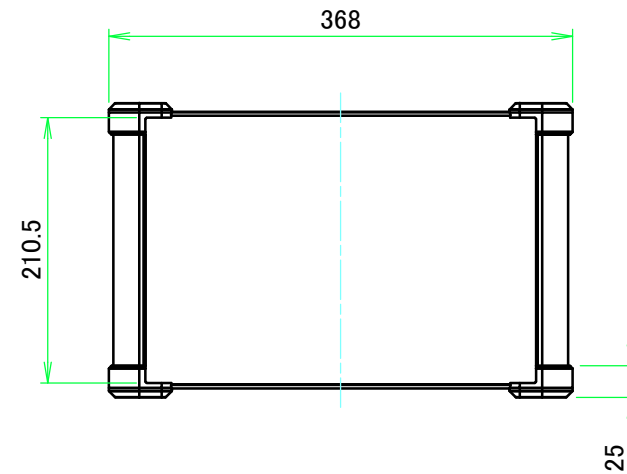
C view
