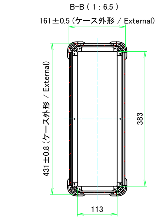
D view
