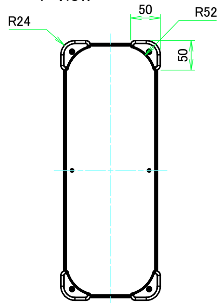
F view
