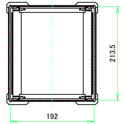
C-C (1:5)
