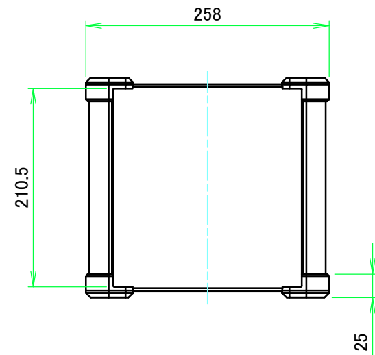
C view
