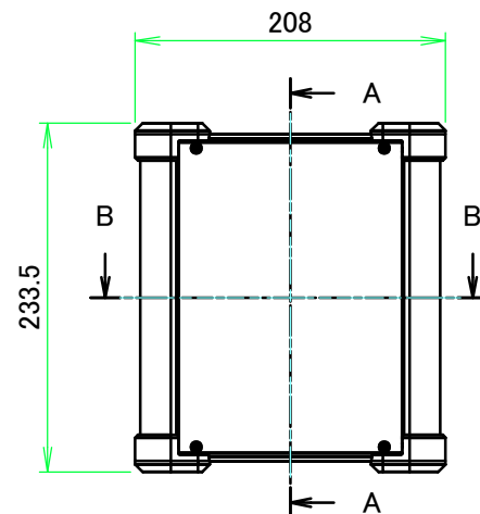
A view
