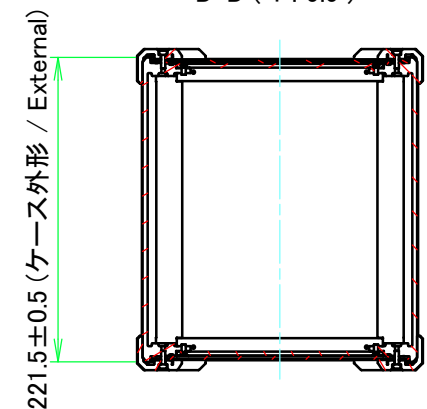
D-D (1:5.5)
