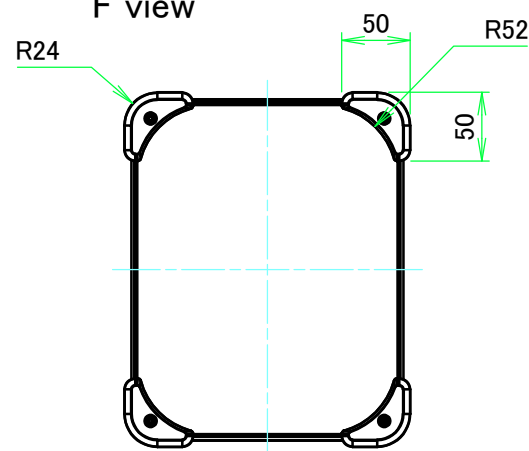
F view
