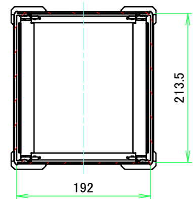
C-C (1:5.5)
