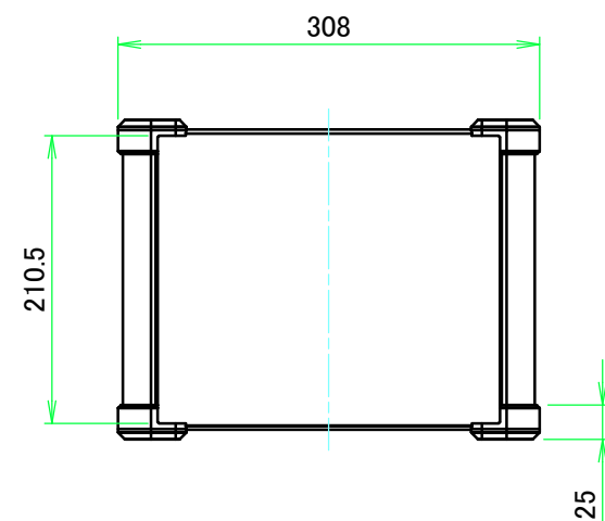
C view
