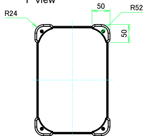
F view
