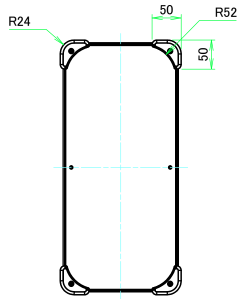
F view
