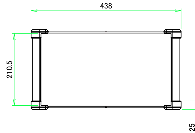
C view
