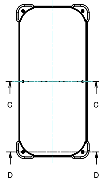
A view
