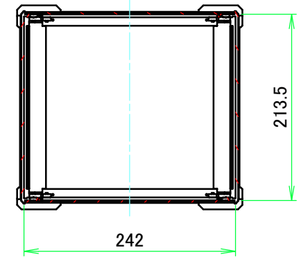
C-C (1:6)
