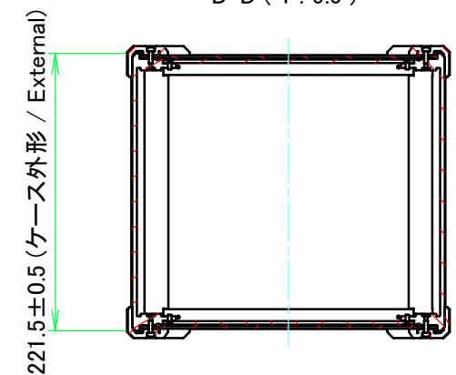
D-D (1:5.5)
