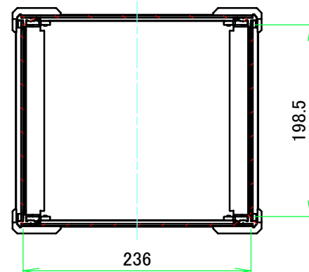
A-A (1:5.5)
