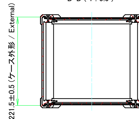
D-D (1:5.5)
