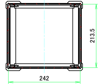
C-C (1:6)
