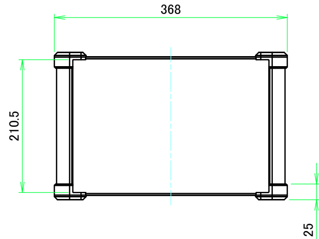
C view
