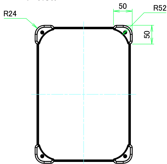
F view
