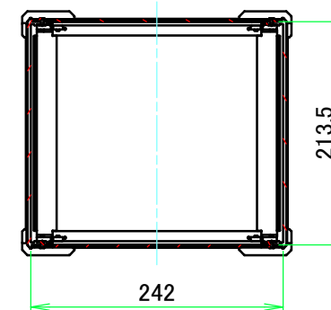
C-C (1:6.5)
