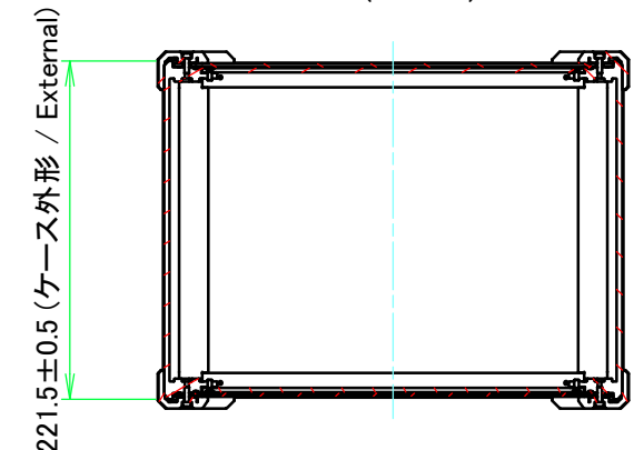
D-D (1:5.5)
