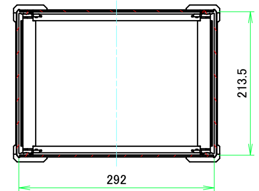
B view
