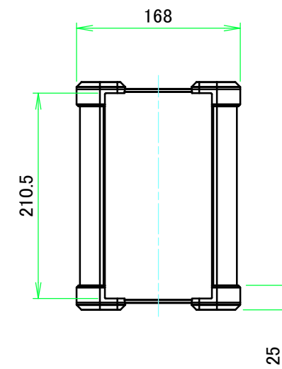
C view
