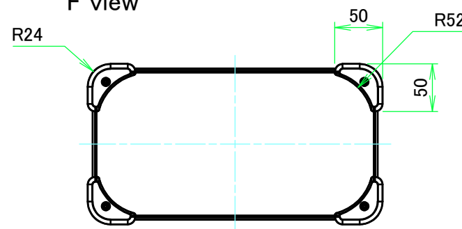
F view
