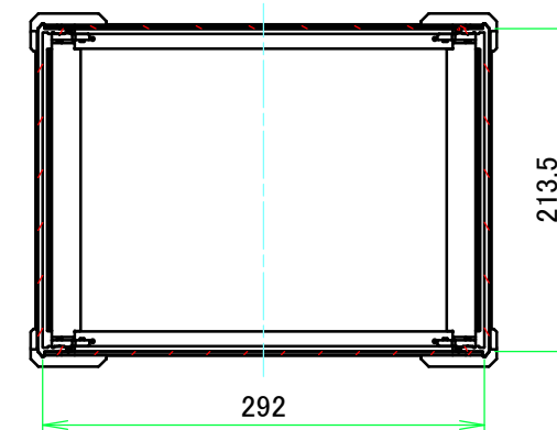
C-C (1:5.5)
