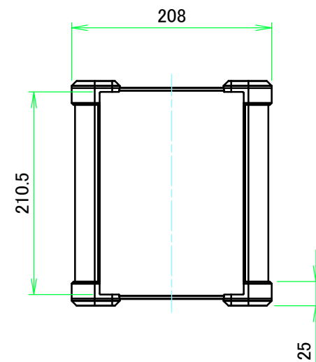
C view
