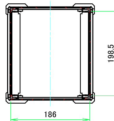
A-A (1:5.5)
