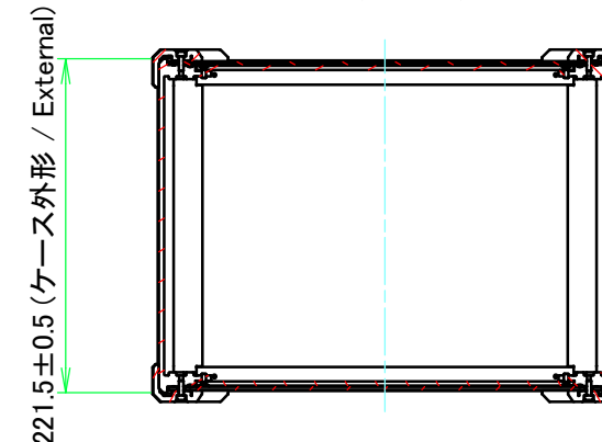
D-D (1:5.5)
