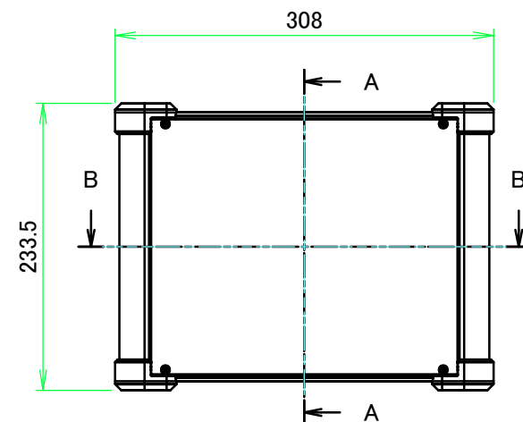
A view
