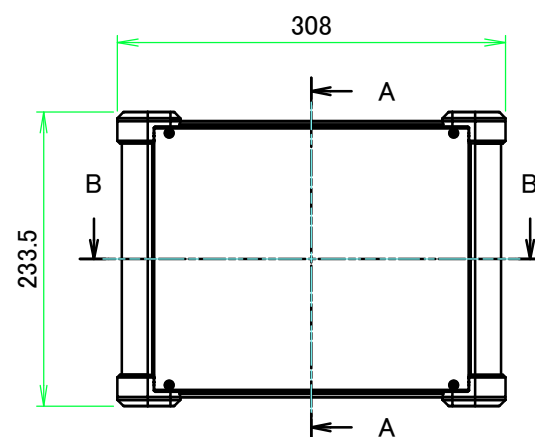
A view
