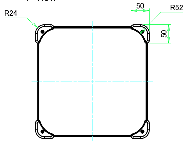
F view
