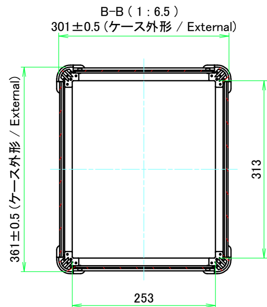
D view
