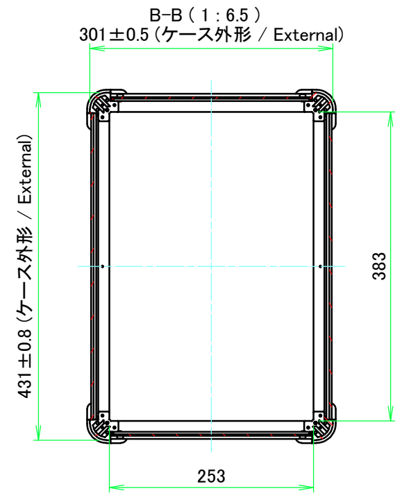
D view
