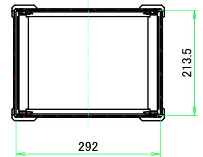
C-C (1:7.5)
