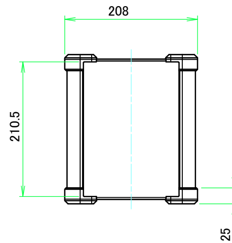
C view
