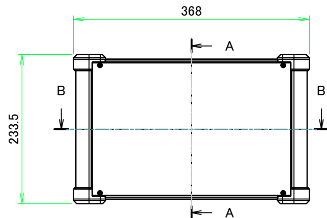
A view
