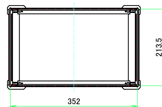
C-C (1:6.5)
