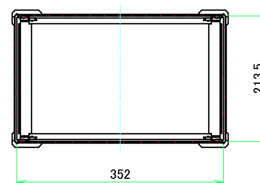
C-C (1:6.5)
