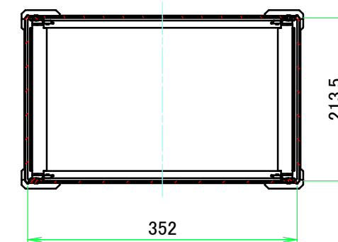
C-C (1:7)
