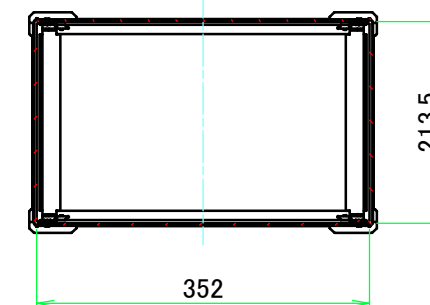
C-C (1:8)
