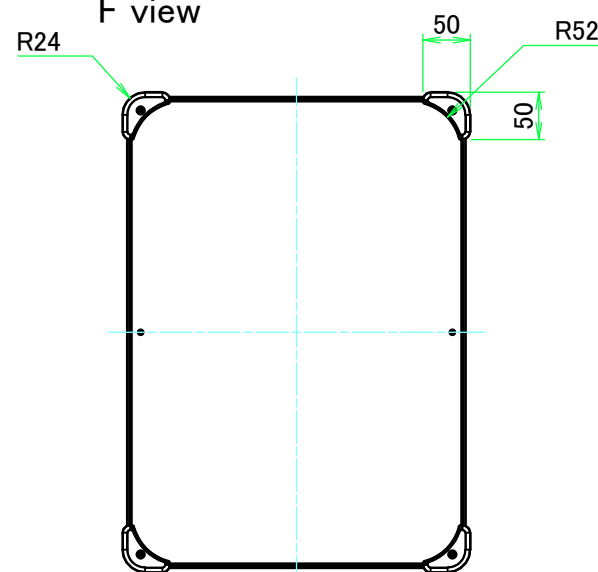
F view
