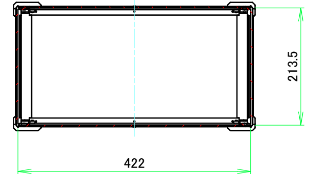
C-C (1:7)
