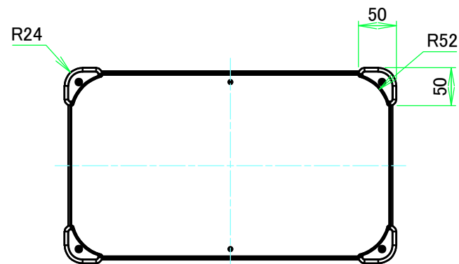
F view
