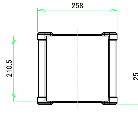
C view
