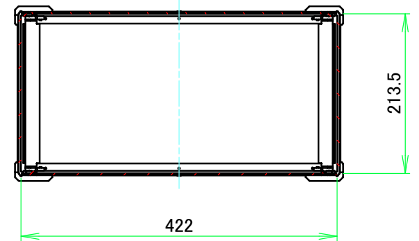
C-C (1:7)
