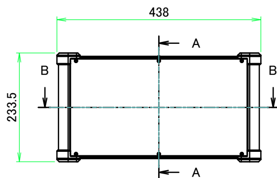
A view
