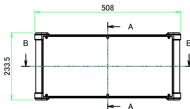
A view
