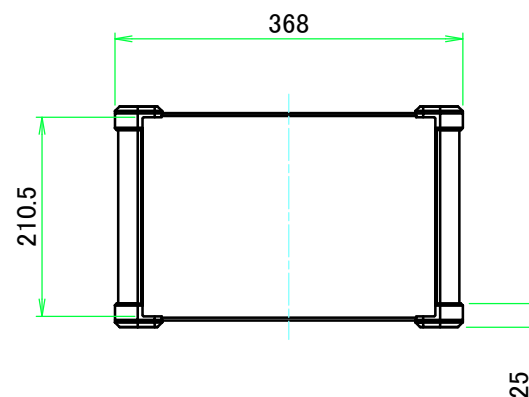
C view
