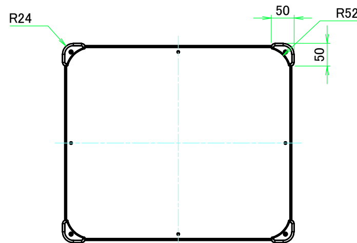
F view
