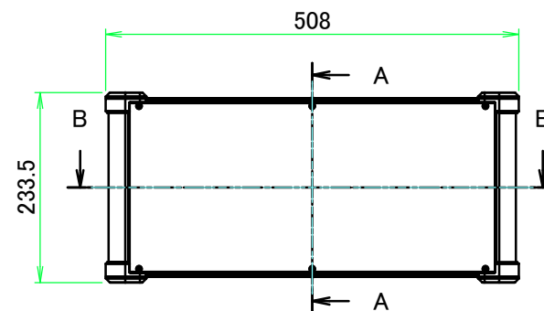
A view
