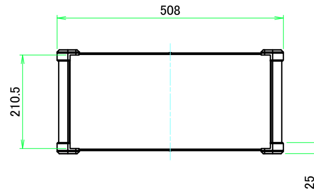
C view
