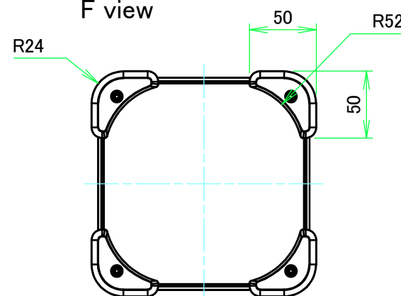
F view
