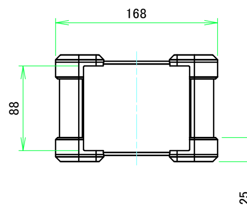
C view
