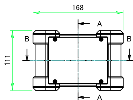
A view
