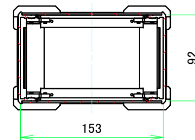
C-C (1:4)
