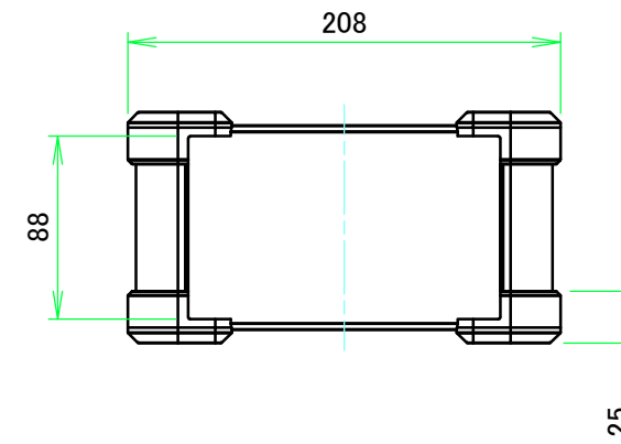
C view
