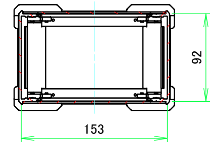
C-C (1:4)
