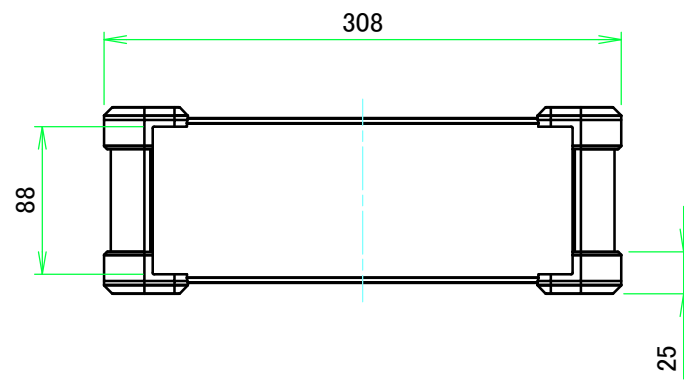
C view
