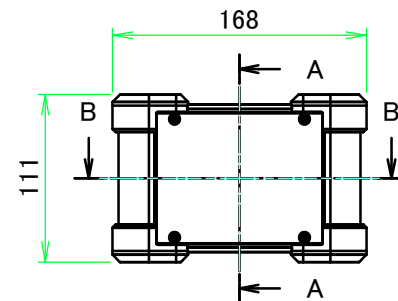
A view
