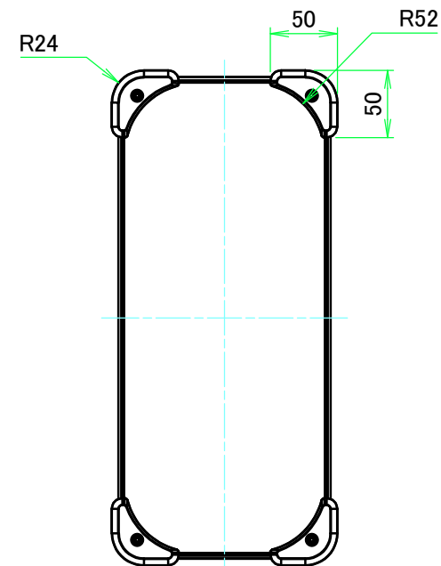
F view
