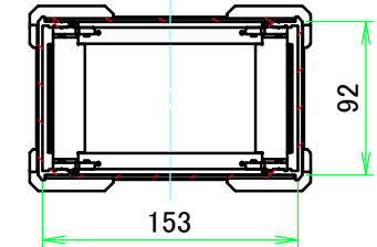
C-C (1:5)
