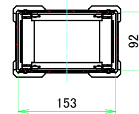
C-C (1:6)
