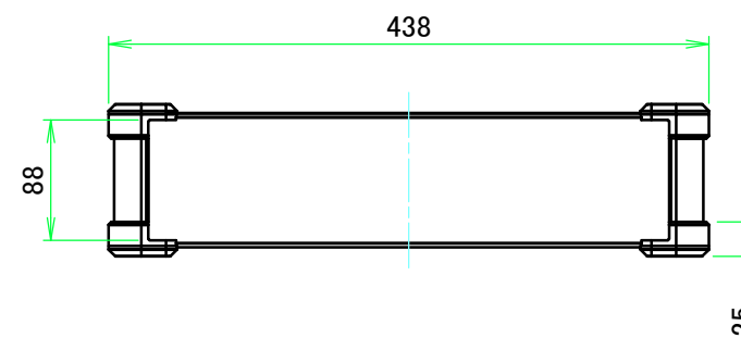
C view
