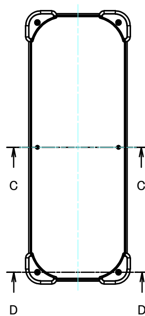
E view
