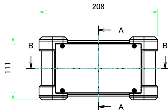
A view
