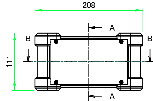
A view
