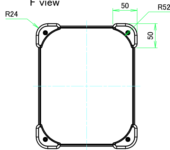
F view
