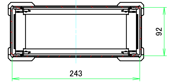
C-C (1:4.5)
