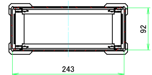
C-C (1:5)
